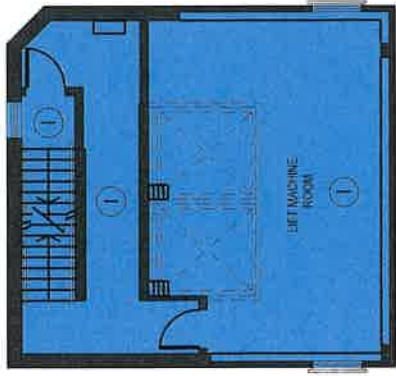
PART PLAN AT LEV. 96.845
