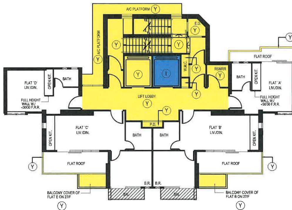
28TH FLOOR PLAN
