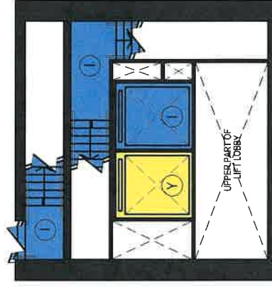
PART PLAN BETWEEN G/F TO 1/F
